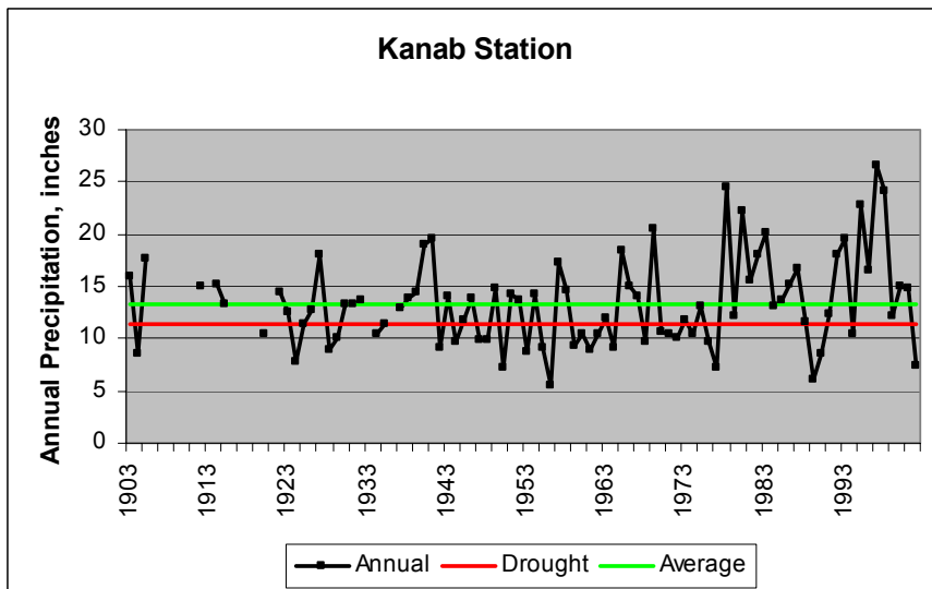
Figure 1. Annual precipitation patterns in Escalante, Kanab and Vernal, Utah
