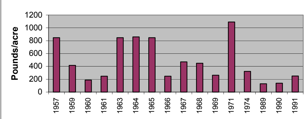
Figure 5. Crested Wheatgrass Production at Malta, Idaho
