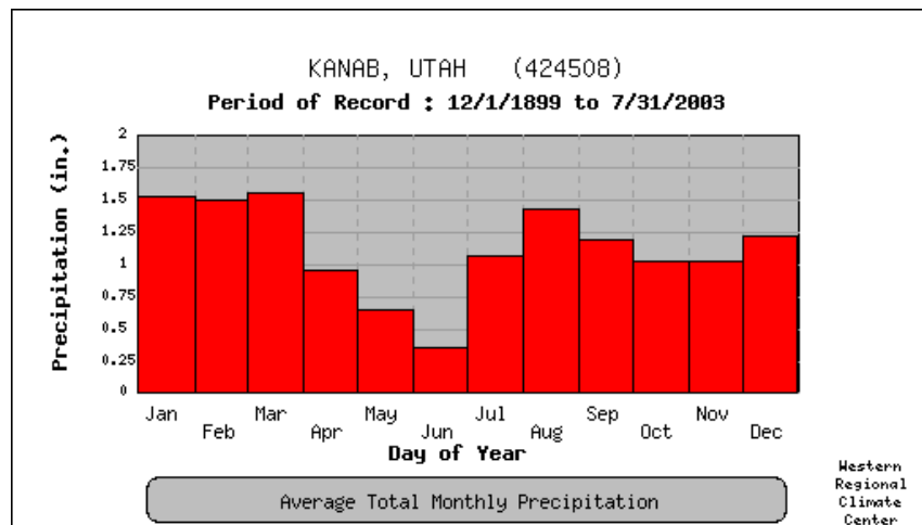
Figure 2. Monthly precipitation patterns in Escalante, Kanab and Vernal, Utah
